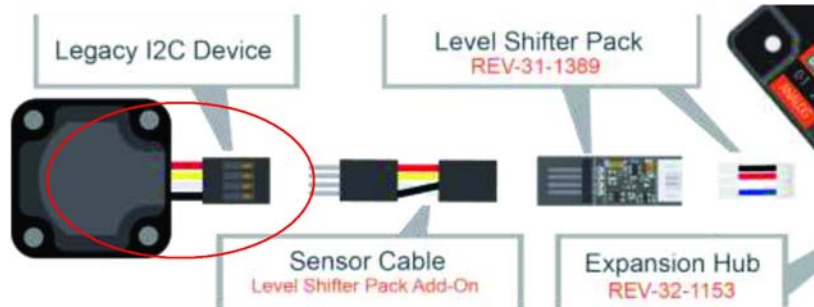
Figure 7: Connecting a Legacy 5V Sensor to an Expansion
