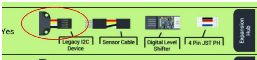
Figure 7: Connecting a Legacy 5V Sensor to an Expansion
